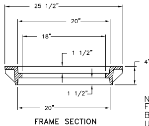
FRAME SECTION
