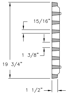
GRATE SECTION
