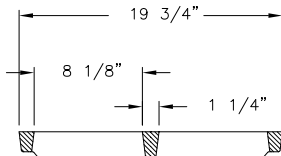
GRATE SECTION
